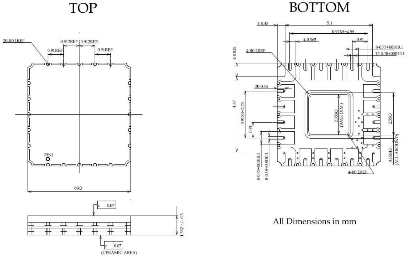
Fig. 8. CQFN44 Package Drawing (All Dimensions in mm)
