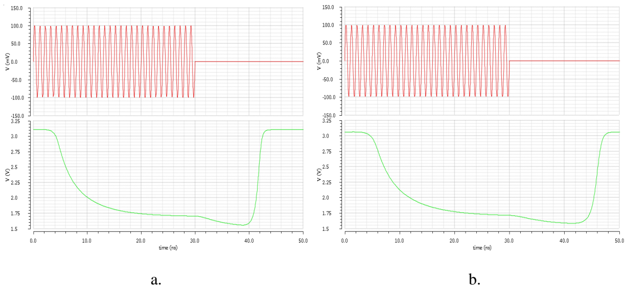
Fig. 6. Peak Detector settling Time (a – Nominal, b – Worst Case Slow)
