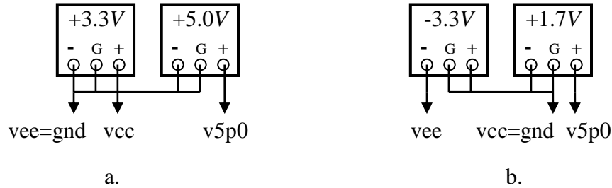
Fig. 2. Power Supply Configurations: Positive (a) and Negative (b)
