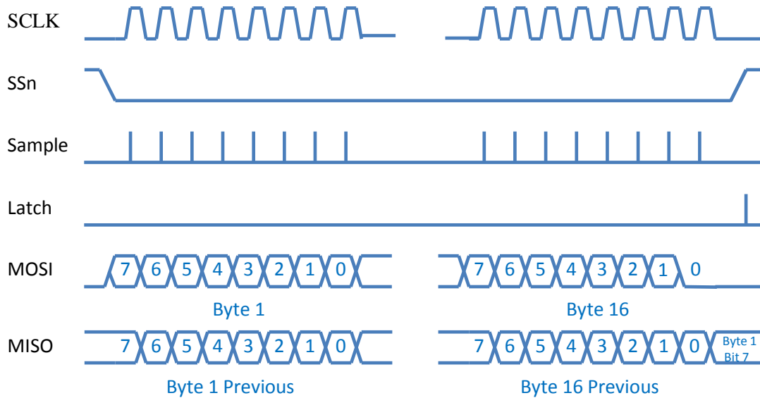
Fig. 7. SPI Timing Diagram
