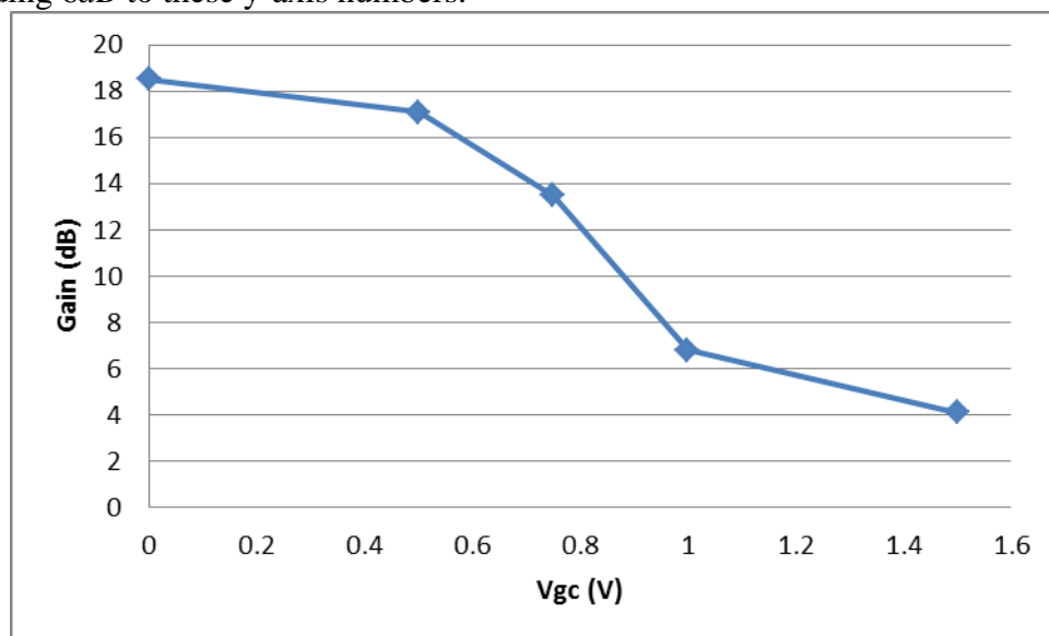
Fig. 2. Single-ended Gain vs. Vgc
