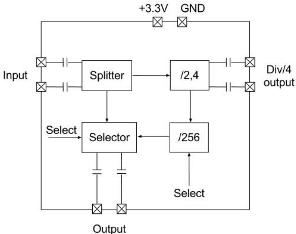
Fig. 5. Functional Block Diagram
