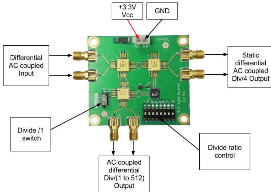
Fig. 2. Terminal Functions Diagram
