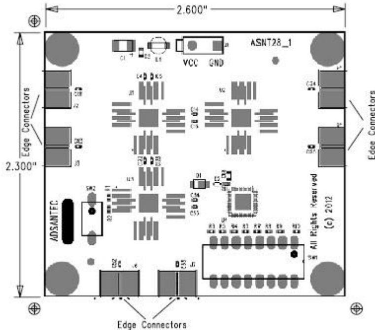
Fig. 6. Board dimensions diagram
