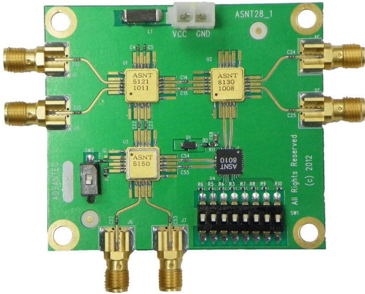
Fig. 1. ASNT28_1 evaluation board
