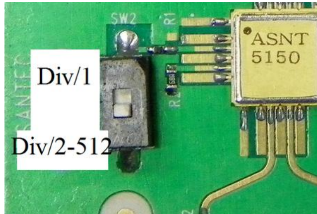
Fig. 4. Divide switch settings
